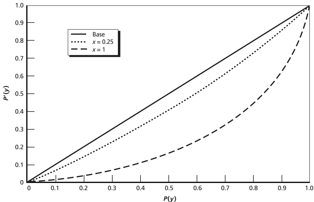
Figure 2.1 Probability Transformation
